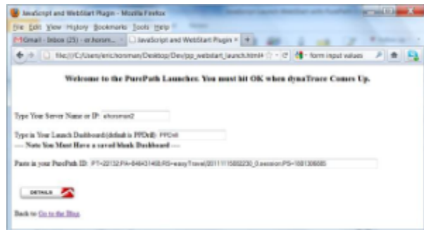
Server, dashboard and PurePath ID specified
